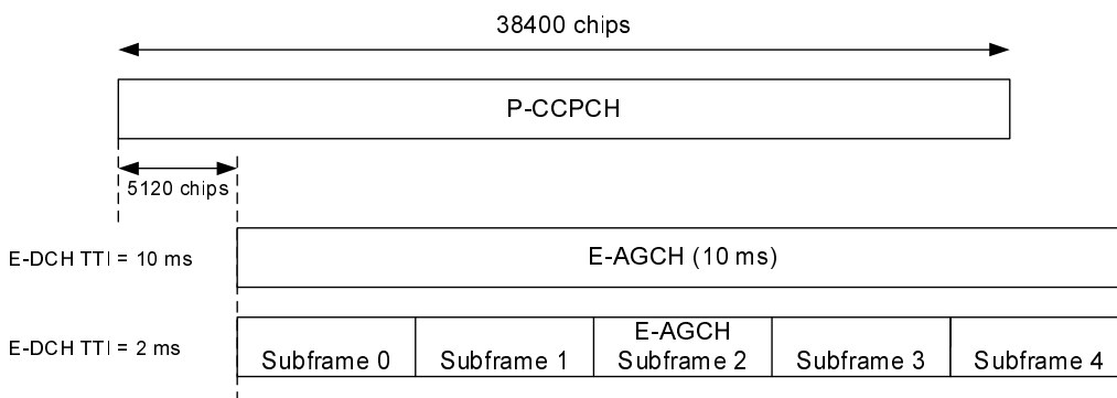
Figure 39: E-AGCH timing
