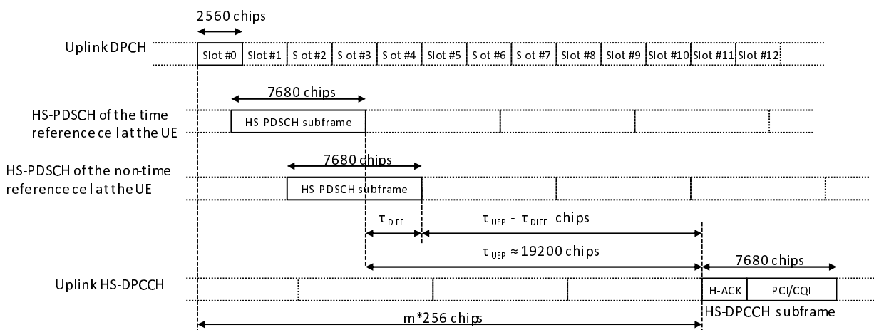
Figure 34a: Timing structure at the UE for HS-DPCCH control signalling with Multiflow, when the UE is not configured in MIMO mode, as well as when the UE is configured in MIMO mode in any cell and the UE indicated not requiring a Longer HARQ processing Time in higher layers
