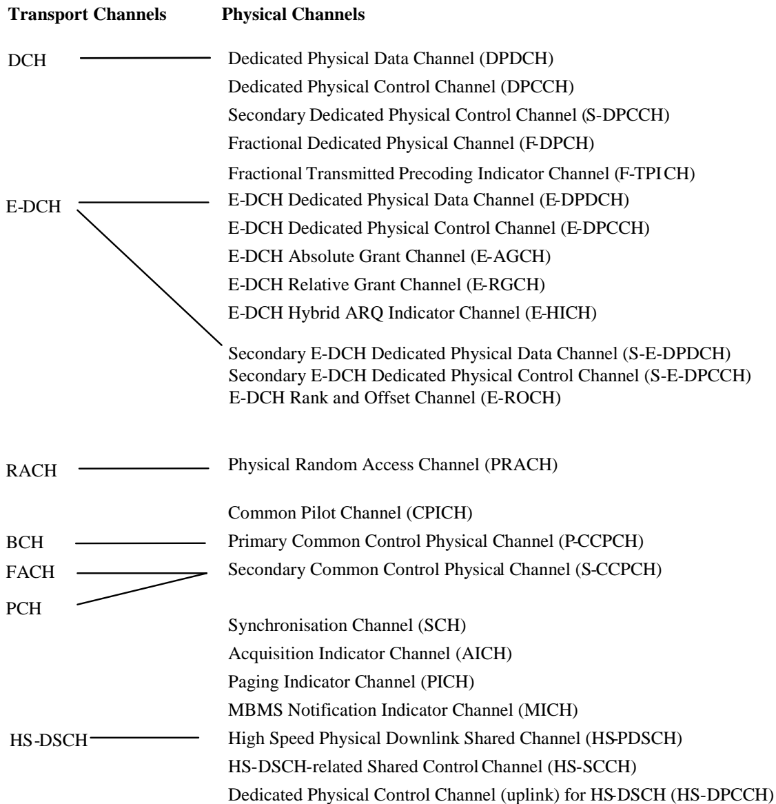
Figure 27: Transport-channel to physical-channel mapping
