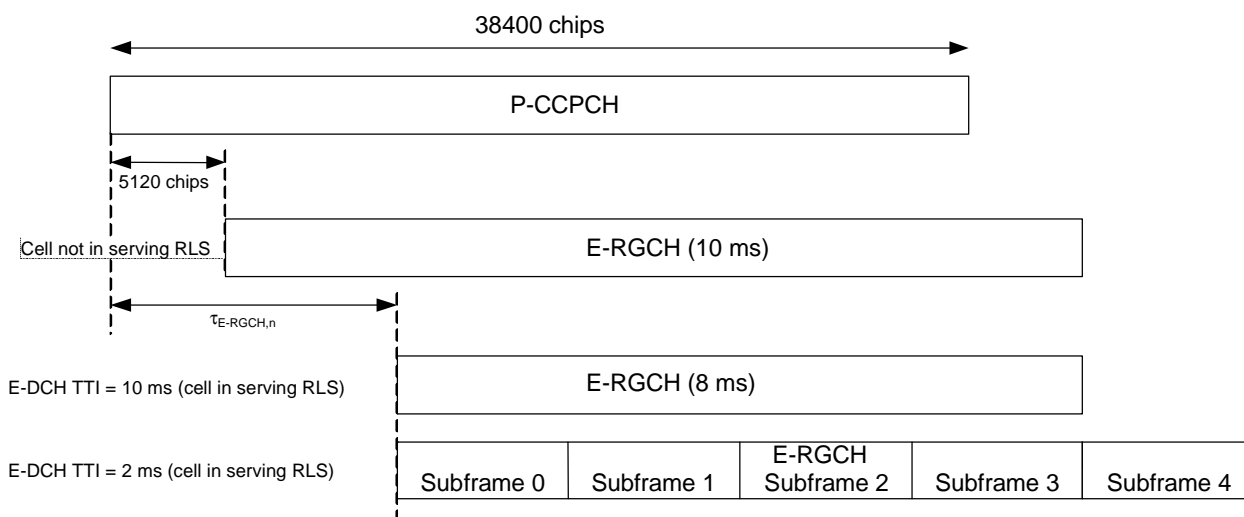
Figure 38: E-RGCH timing
