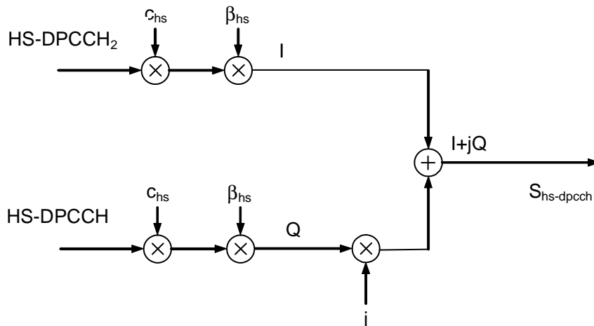
Figure 1B.1: Spreading for uplink HS-DPCCHs when Secondary_Cell_Enabled is greater than 3
