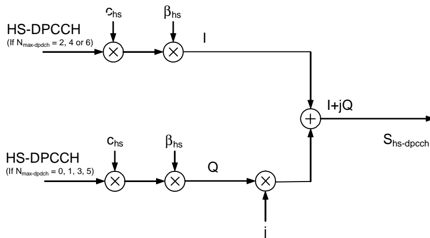
Figure 1B: Spreading for uplink HS-DPCCH when Secondary_Cell_Enabled is less than 4
