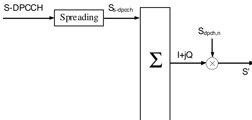
Figure 1.1: Spreading for uplink S-DPCCH when UL_CLTD_Enabled is TRUE and UL_CLTD_Active=1
