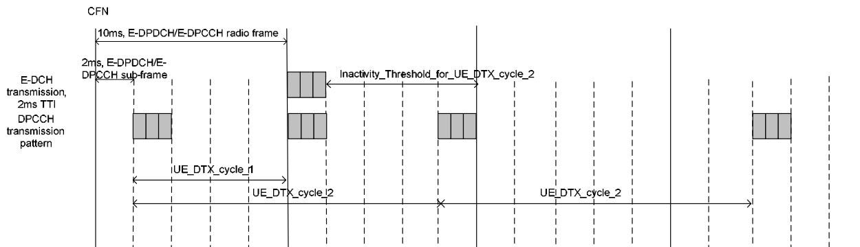
Figure 2A: Example for UL DPCCH discontinuous transmission pattern for 2ms E-DCH TTI beginning at CFN=1 (with UE\_DTX\_DRX\_Offset = 6 )
