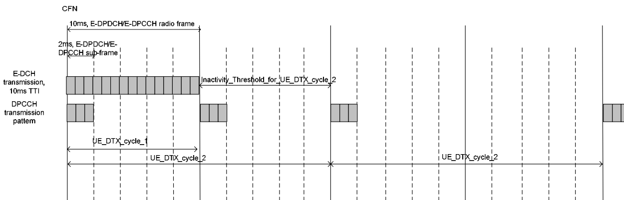
Figure 2B: Example for UL DPCCH discontinuous transmission pattern for 10ms E-DCH TTI beginning at CFN=1 (with UE\_DTX\_DRX\_Offset = 5 )
