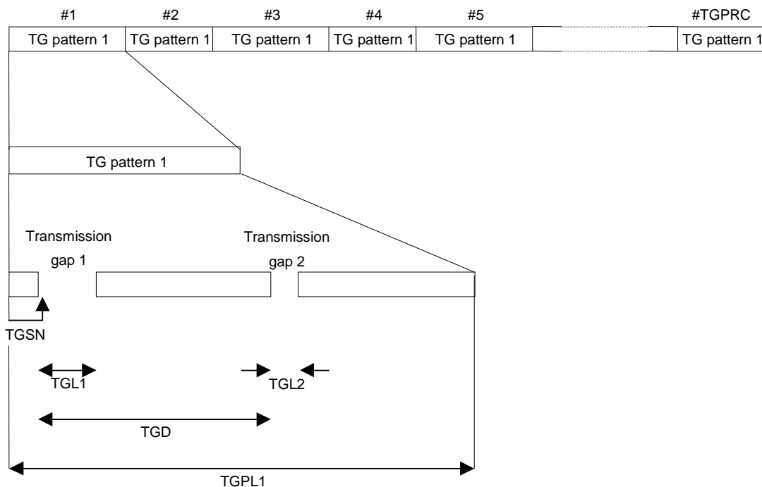
Figure 1: Illustration of compressed mode pattern parameters
