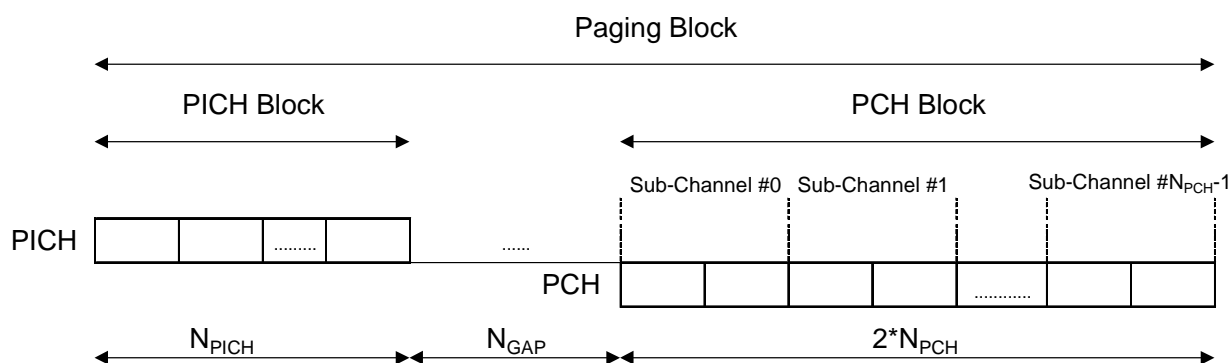
Figure 32: Paging Sub-Channels and Association of PICH and PCH blocks
