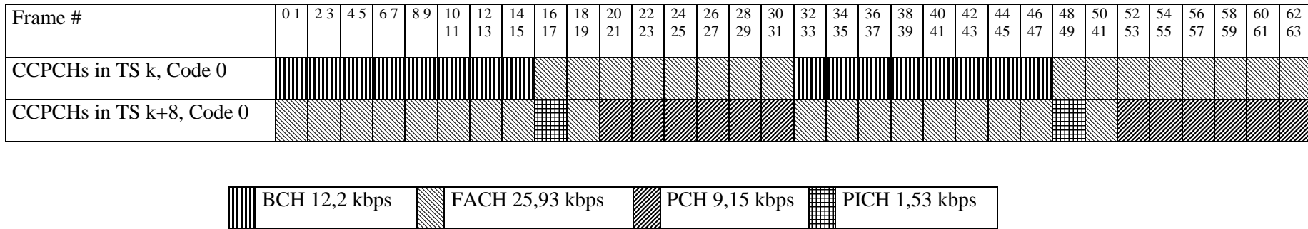
Figure C.1: Example for a multiframe structure for CCPCHs and PICH that is repeated every 64th frame
