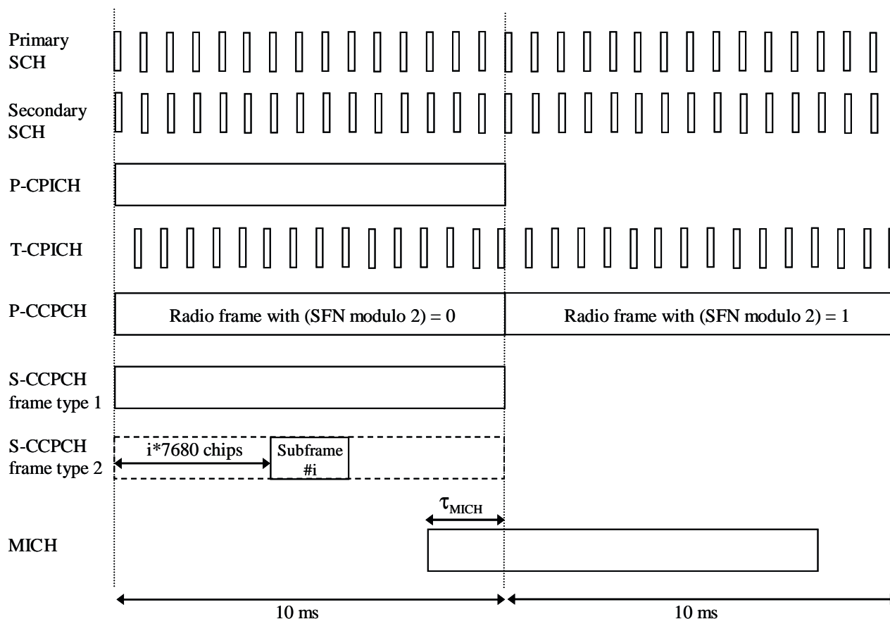
Figure x9: Radio frame and sub-frame timing of downlink physical channels
