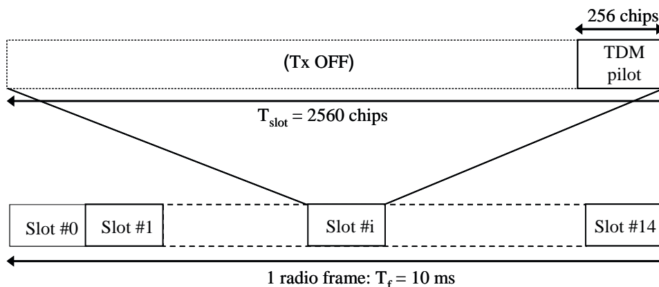
Figure x3: Structure of the Time-multiplexed Common Pilot Channel (T-CPICH)
