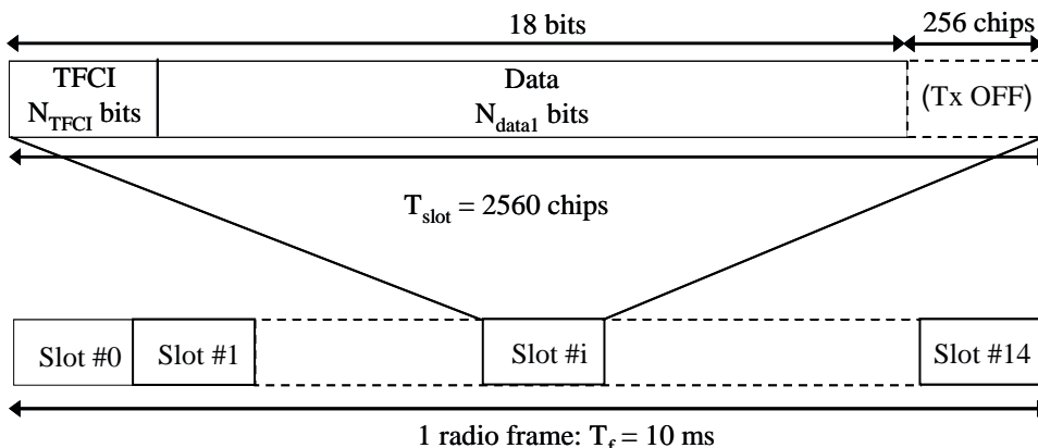
Figure x5: Frame structure for Secondary Common Control Physical Channel frame type 1
