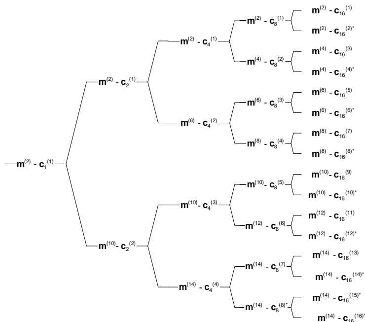
Figure AA.3.2b: Association of Midambles to Spreading Codes for K=14 pattern 2
