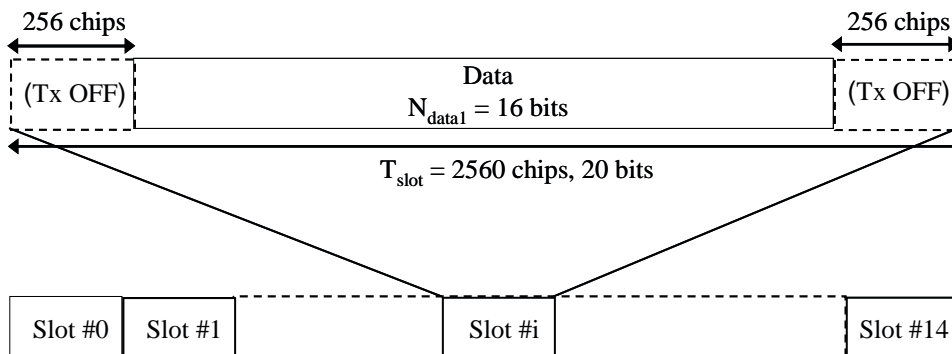
Figure x4: Frame structure for Primary Common Control Physical Channel
