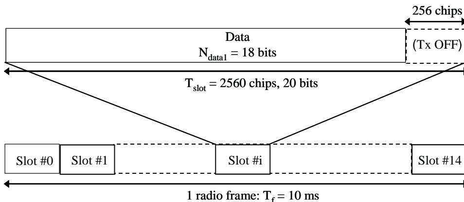
Figure x8: Frame structure for the MBMS Indicator Channel (MICH)
