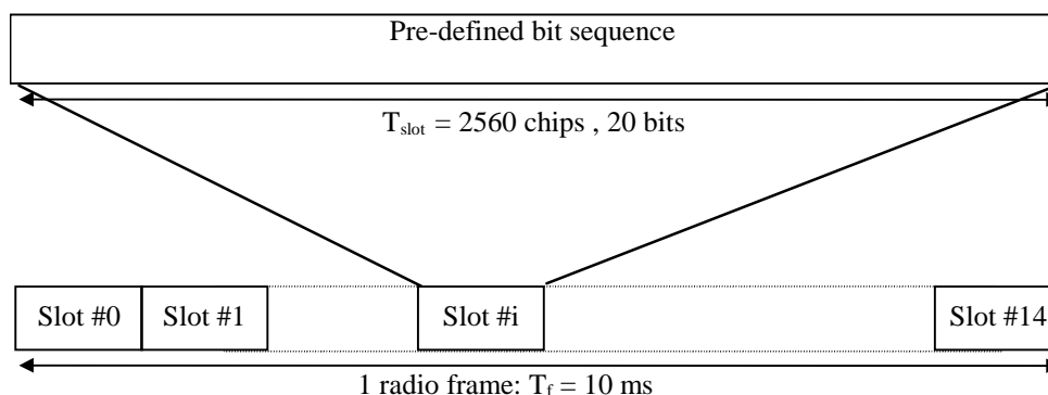
Figure x2: Frame structure for Primary Common Pilot Channel
