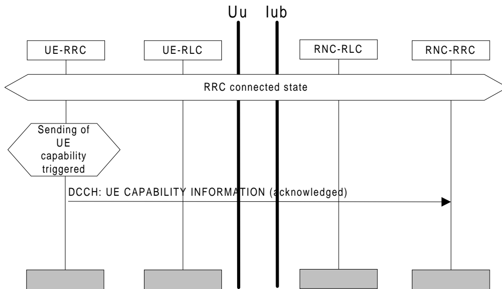
Figure 39: UE Capability Information
