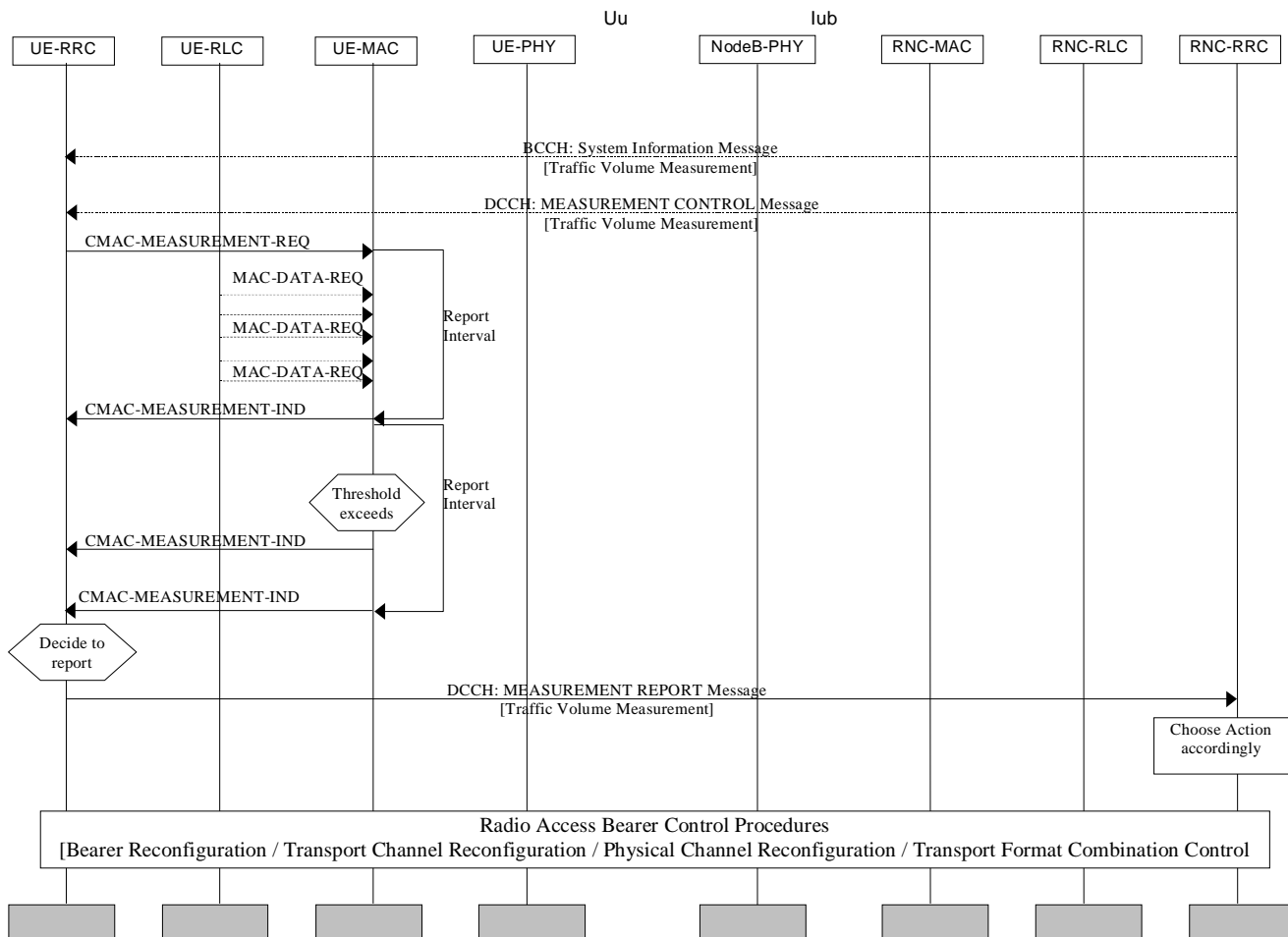
Figure 42: Traffic Volume Measurement Report Procedure
