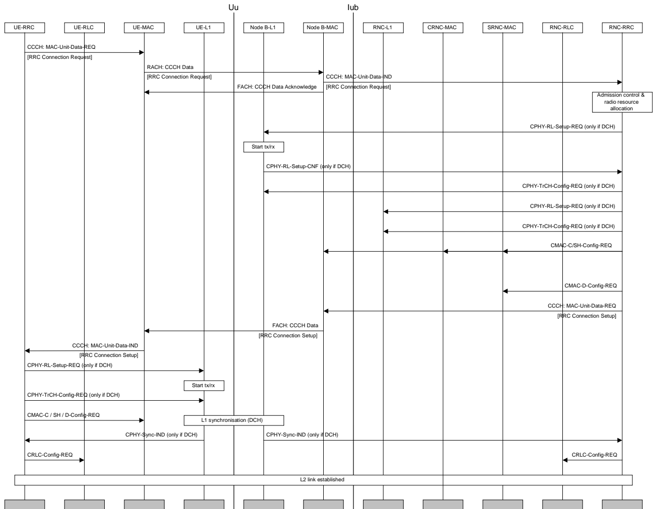
Figure A.1: RRC connection establishment with common channel termination case C
