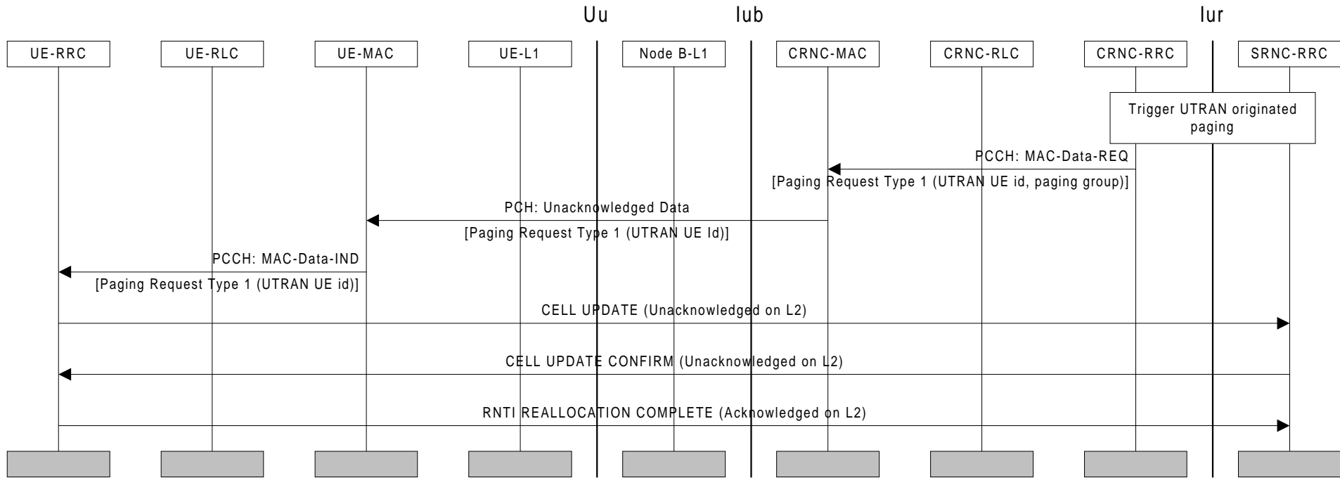
Figure 38: Example sequence for UTRAN initiated paging request with paging response
