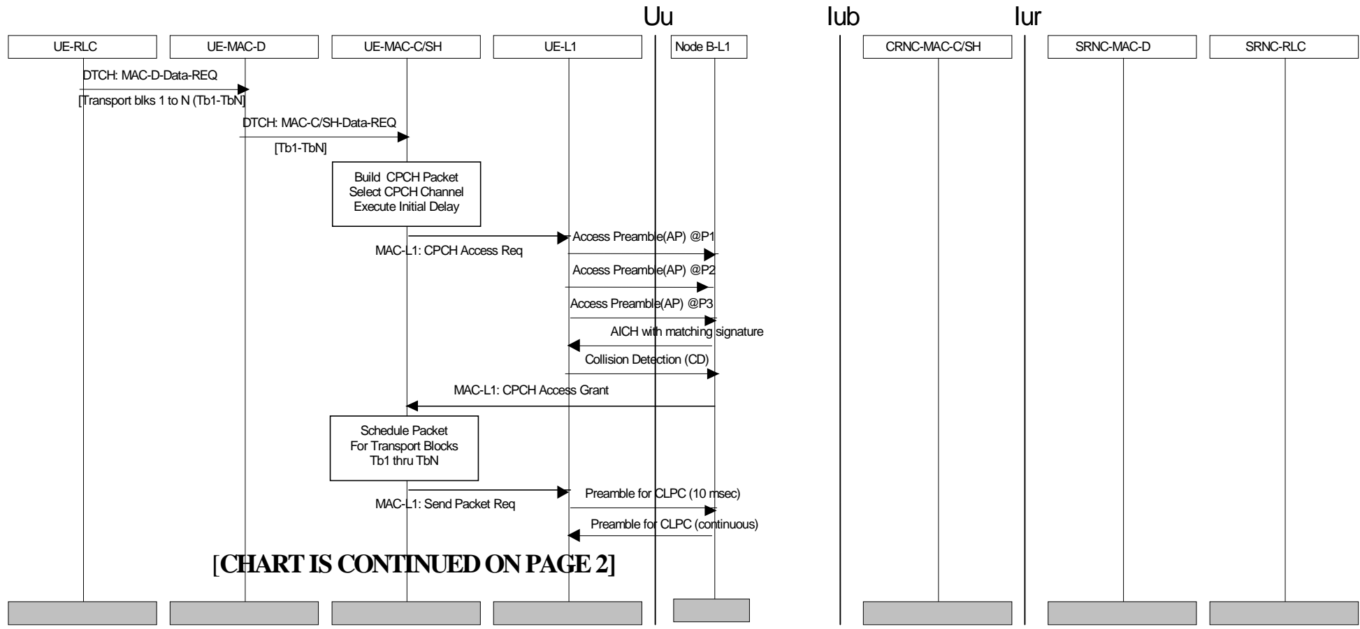
Figure 21: Example of acknowledged-mode data transmission on CPCH (page 1 of 2)
