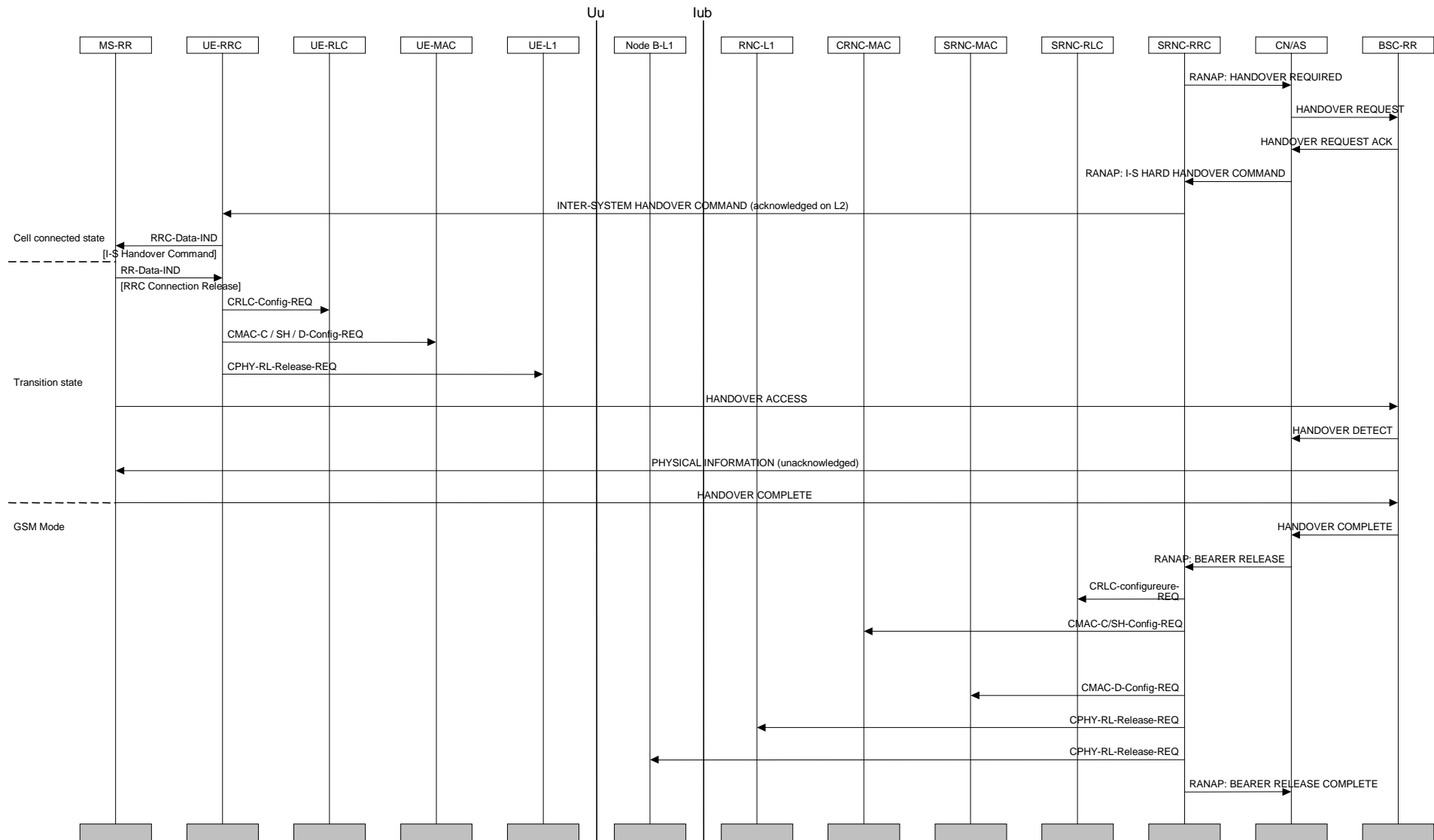
Figure 36: UMTS to GSM inter-system handover
