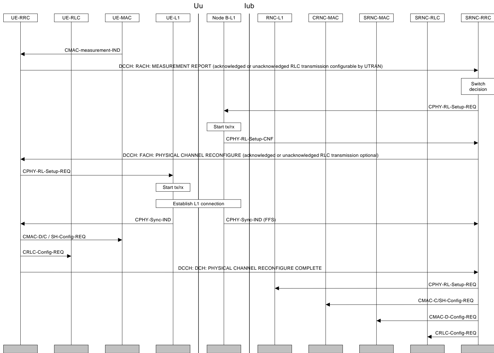
Figure 14: UE-Originated DCH Activation
