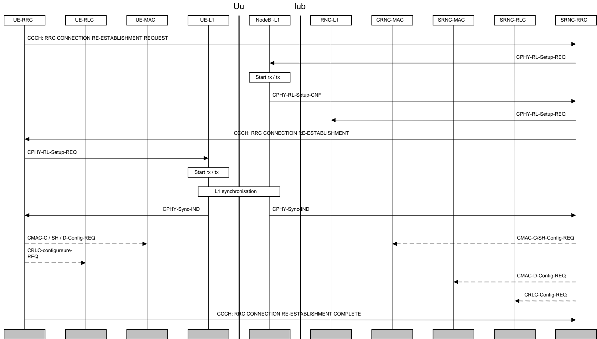
Figure 34: RRC connection re-establishment
