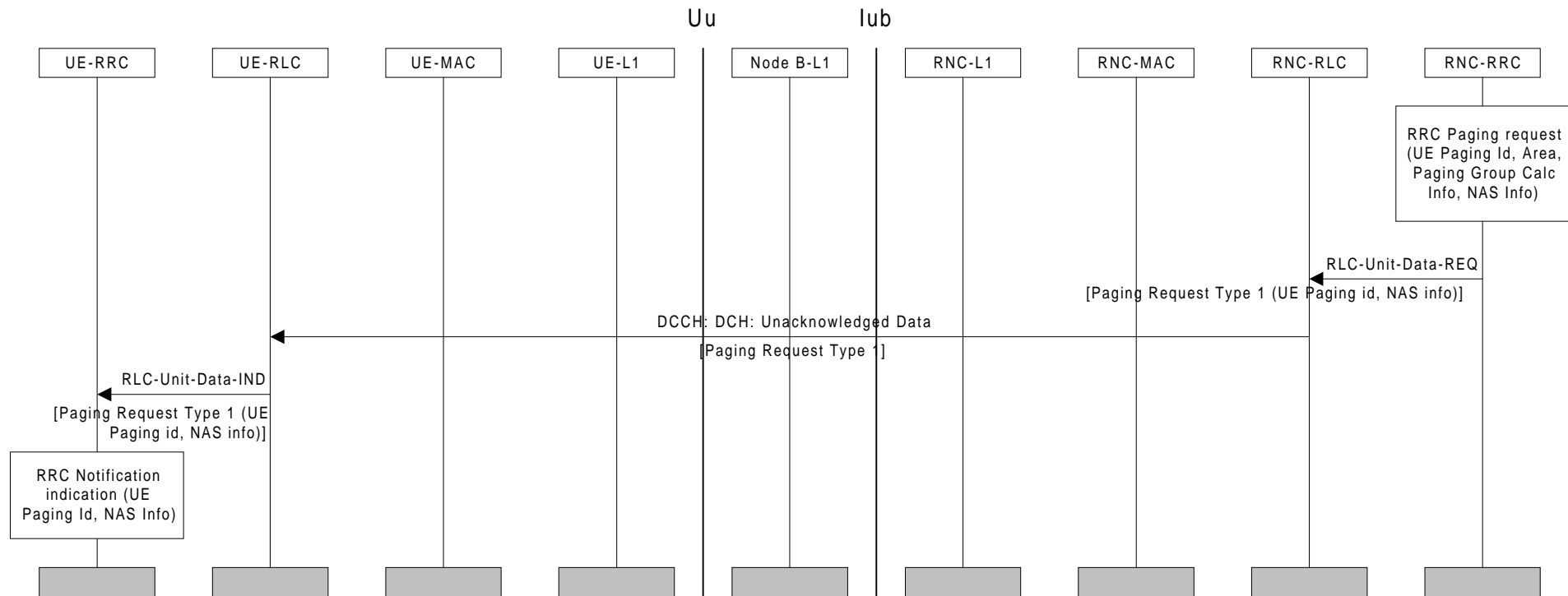
Figure 37. Example sequence of CN initiated paging request using DCCH
