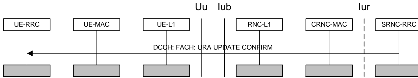
Figure 28: Case A continuation of URA update, CONFIRM message can be ciphered
