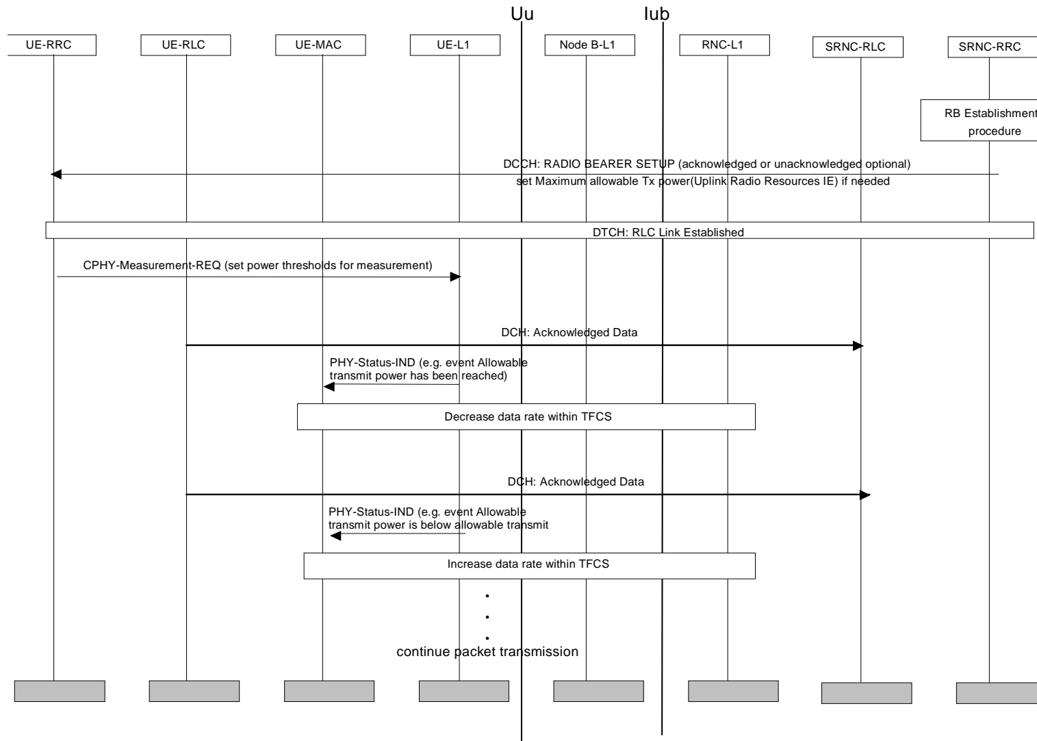
Figure 18: Variable Rate Transmission of Uplink DCHs
