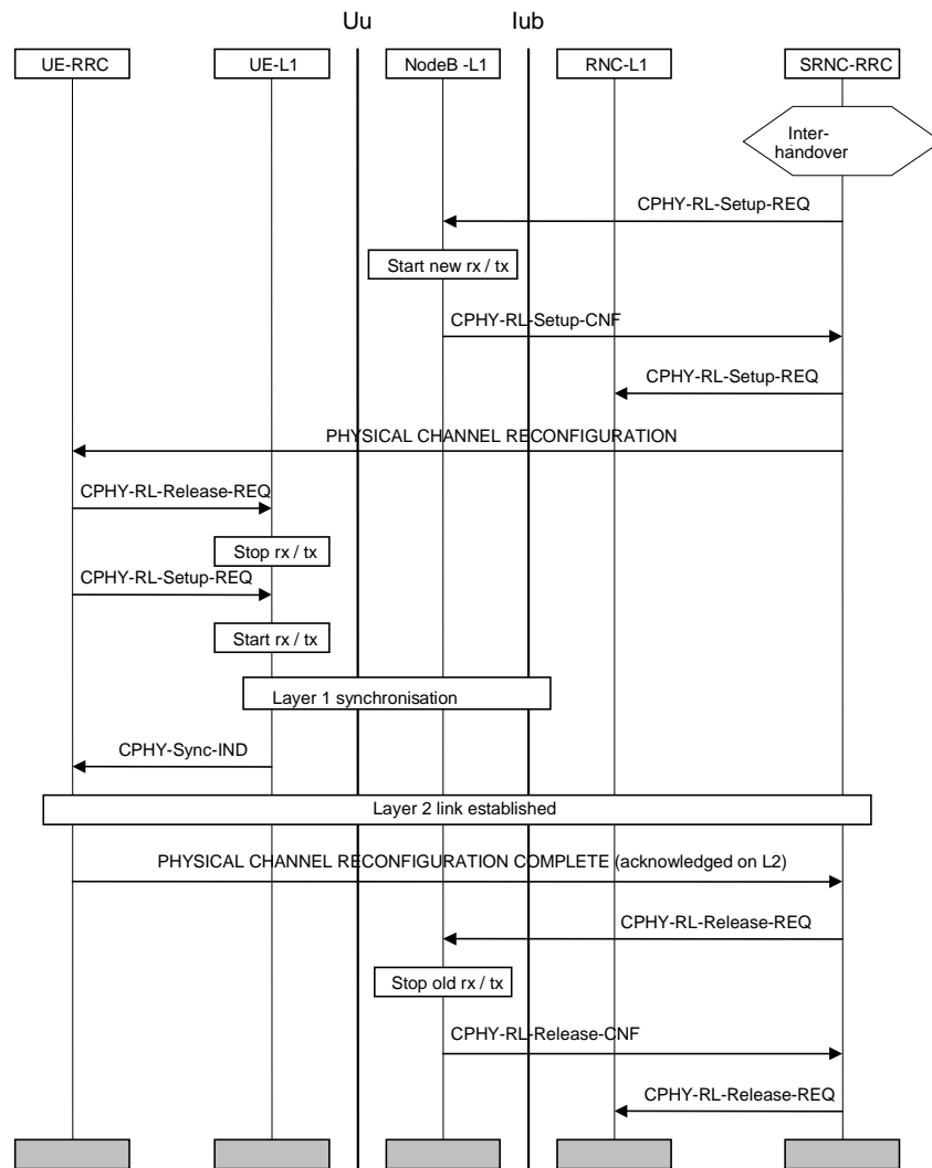
Figure 33: Hard handover
