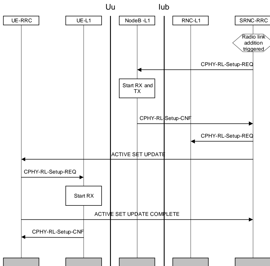
Figure 30: Radio Link Addition
