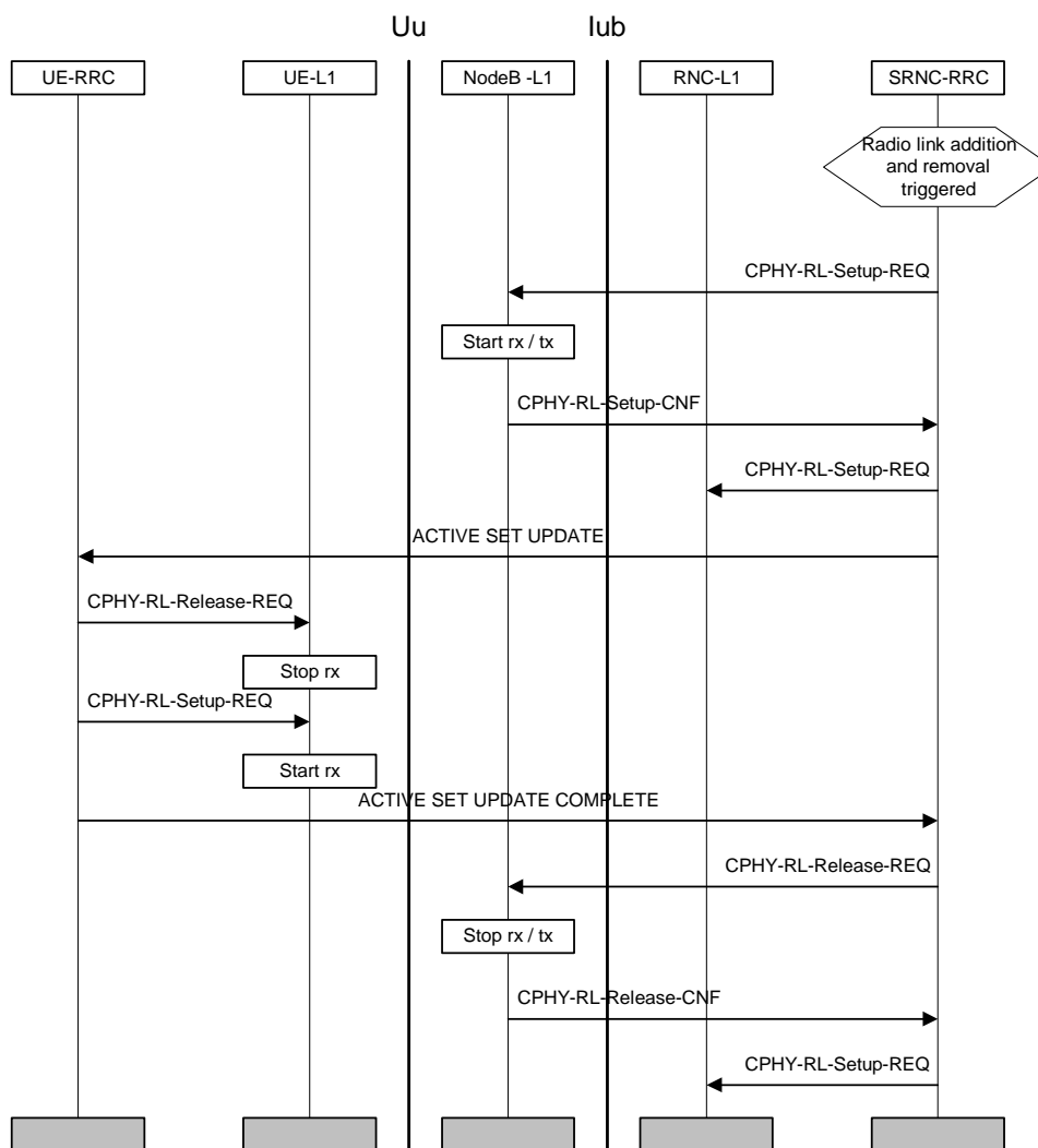
Figure 32: Combined Radio Link Addition And Removal
