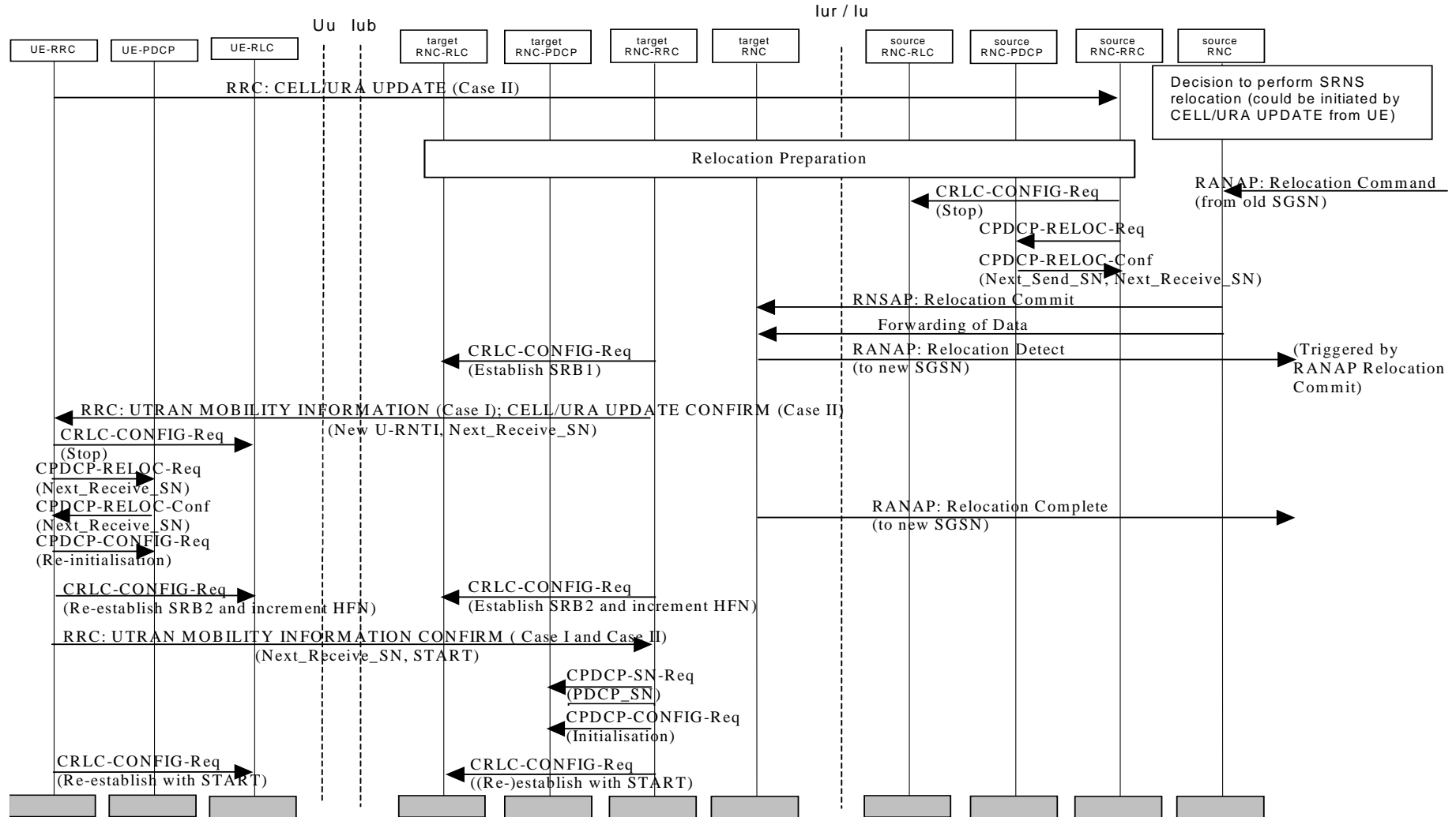
Figure 34: Combined Cell/URA Update and SRNS relocation (lossless radio bearers)
