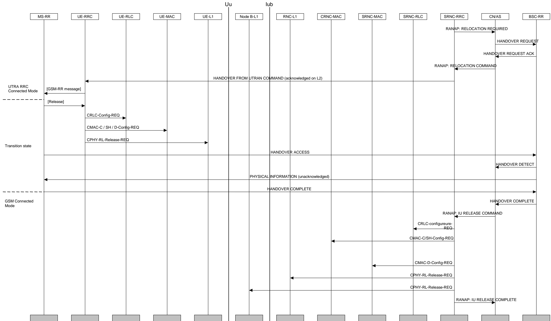
Figure 40: UTRAN to GSM inter-RAT handover
