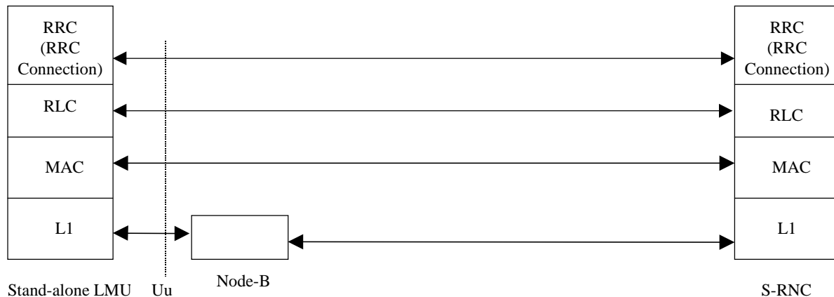
Figure 6.5: Signalling between an RNC and a Stand-Alone LMU using a signalling bearer
