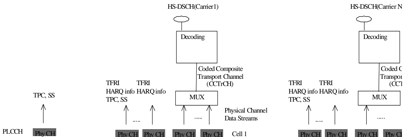
Figure 5.2.2.2-3: Model of the UE's physical layer (1.28Mcps TDD multi-frequency HS-DSCH operation mode only)
