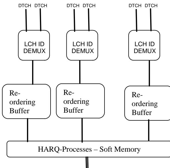
Figure 6.1.2-3: Simplified architecture showing MAC-es inter-working in UE
