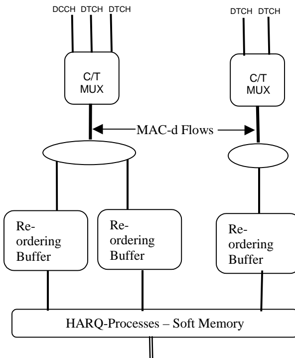
Figure 6.1.2-2: Simplified architecture showing MAC-ds inter-working in UE
