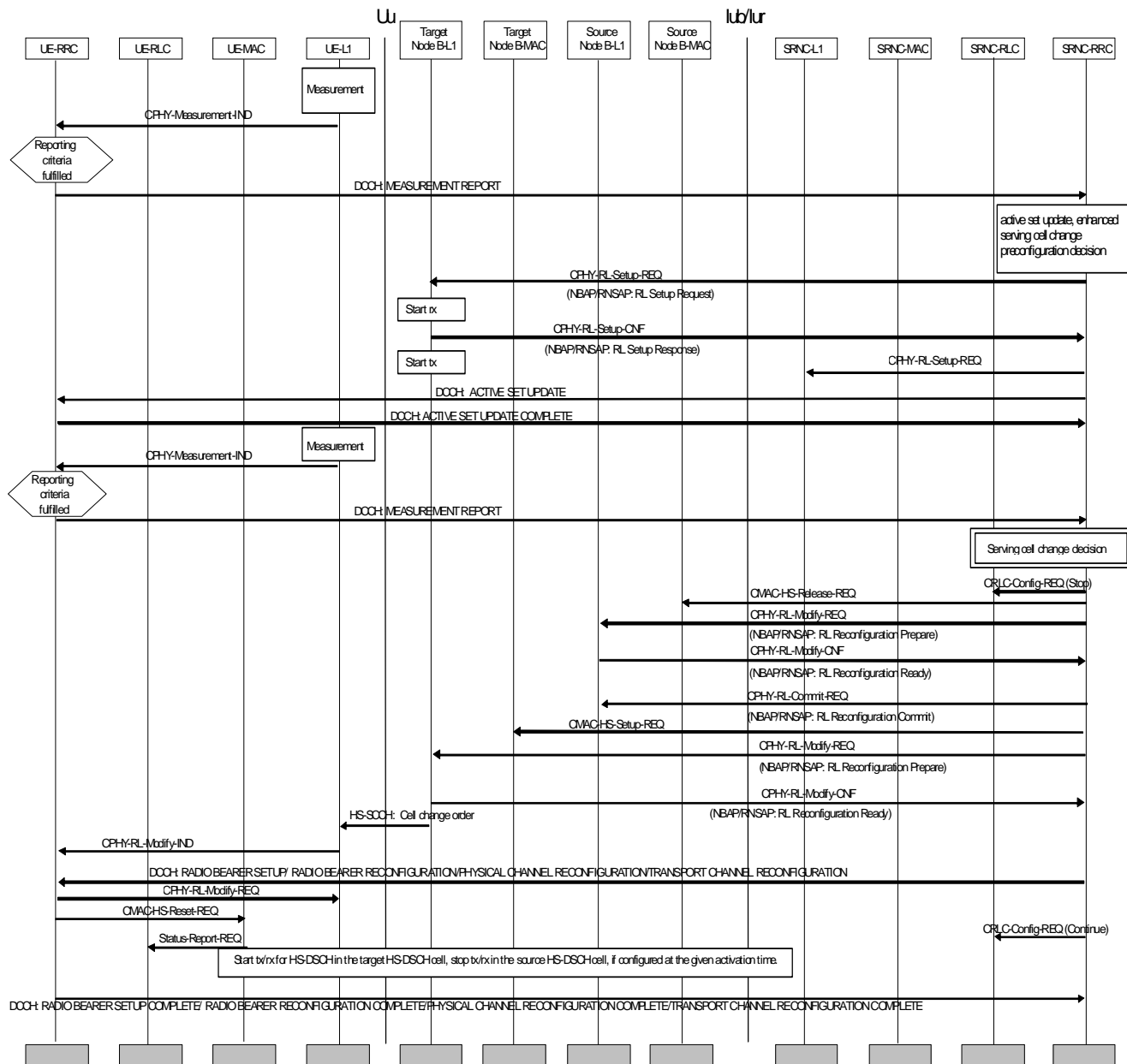
Figure 9.6-1: Inter-Node B serving HS-DSCH cell change with target cell pre-configuration
