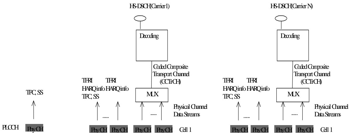
Figure 5.2.2.2-3: Model of the UE's physical layer in CELL_DCH state (1.28Mcps TDD multi-frequency HS-DSCH operation mode only)
