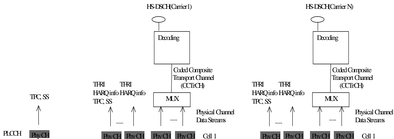
Figure 5.2.2-3: Model of the UE's physical layer in CELL_DCH state (1.28Mcps TDD multi-frequency HS-DSCH operation mode only)
