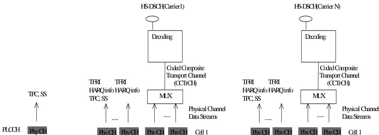
Figure 5.2.2.2-3: Model of the UE's physical layer in CELL_DCH state (1.28Mcps TDD multi-frequency HS-DSCH operation mode only)
