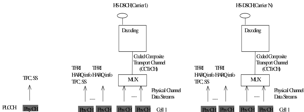
Figure 5.2.2.2-3: Model of the UE's physical layer in CELL_DCH state (1.28Mcps TDD multi-frequency HS-DSCH operation mode only)
