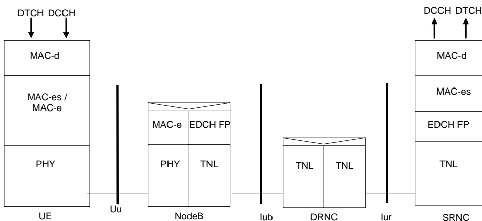
Figure 6.1-1: Protocol Architecture of E-DCH
