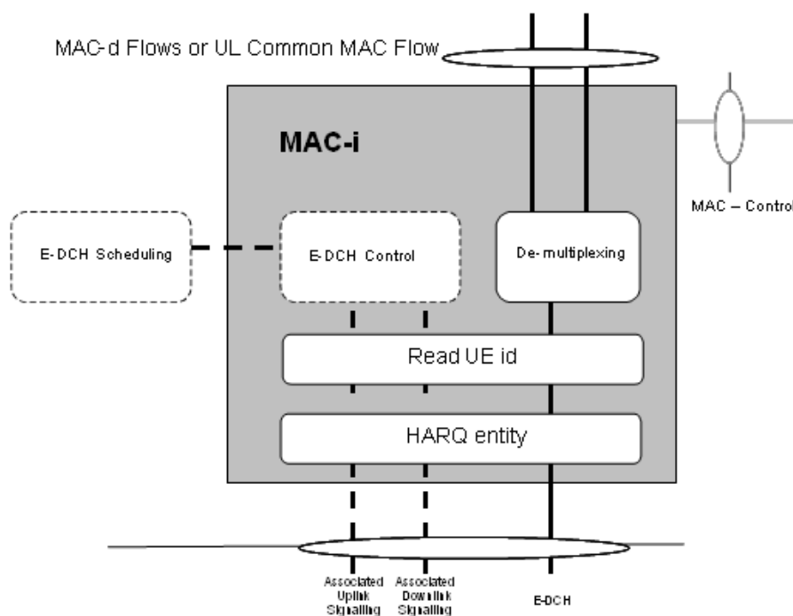
Figure 7.3.8-1: UTRAN side MAC architecture / MAC-i details (FDD only)
