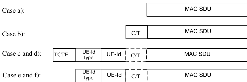
Figure 9.2.1.1.1: MAC PDU formats for DTCH and DCCH
