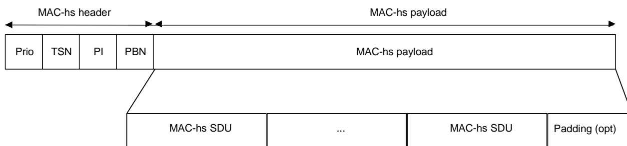
Figure 9.1.4.1: MAC-hs PDU
