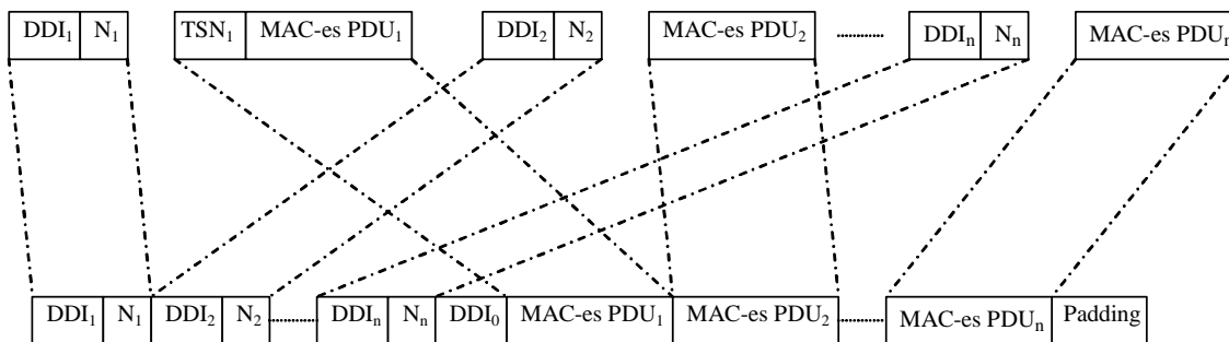
Figure 9.1.5.2: MAC-e PDU
