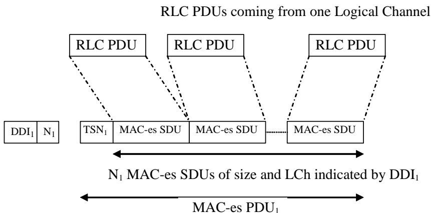
Figure 9.1.5.1: MAC-es PDU
