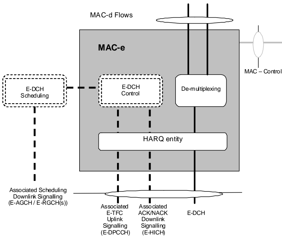
Figure 4.2.4.5-1a: UTRAN side MAC architecture / MAC-e details (FDD)
