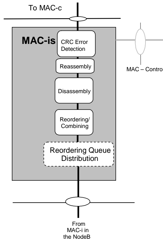
Figure 4.2.4.7-3: UTRAN side MAC architecture / MAC-is details (for CCCH transmission, FDD only)
