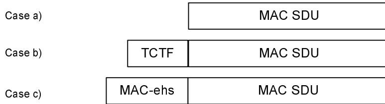
Figure 9.2.1.2.1: MAC PDU formats for BCCH
