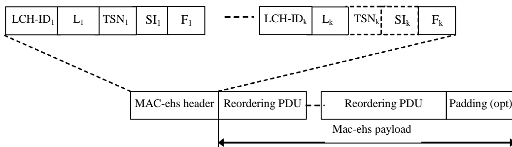
Figure 9.1.4.2: MAC-ehs PDU
