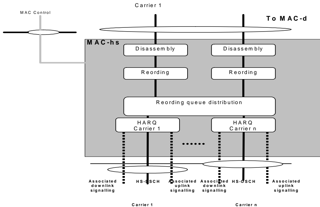
Figure 4.2.3.3.2: UE side MAC architecture/MAC-hs details (1.28Mcps TDD multi-frequency HS-DSCH operation mode only)
