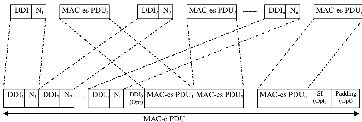
Figure 9.1.5.2a: MAC-e PDU
