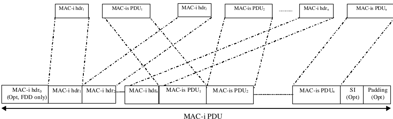
Figure 9.1.5.3 MAC-is PDU.
