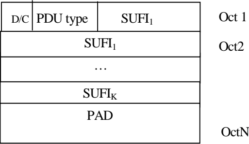
Figure 9.4: STATUS PDU
