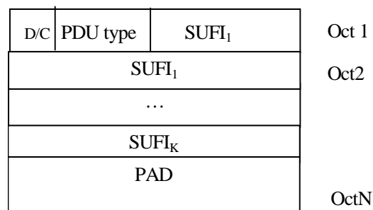
Figure 9.4: STATUS PDU
