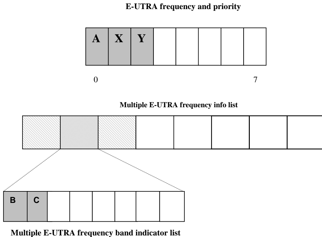
Figure: G.3.1 – Mapping of EARFCN's to Multiple E-UTRA frequency info
