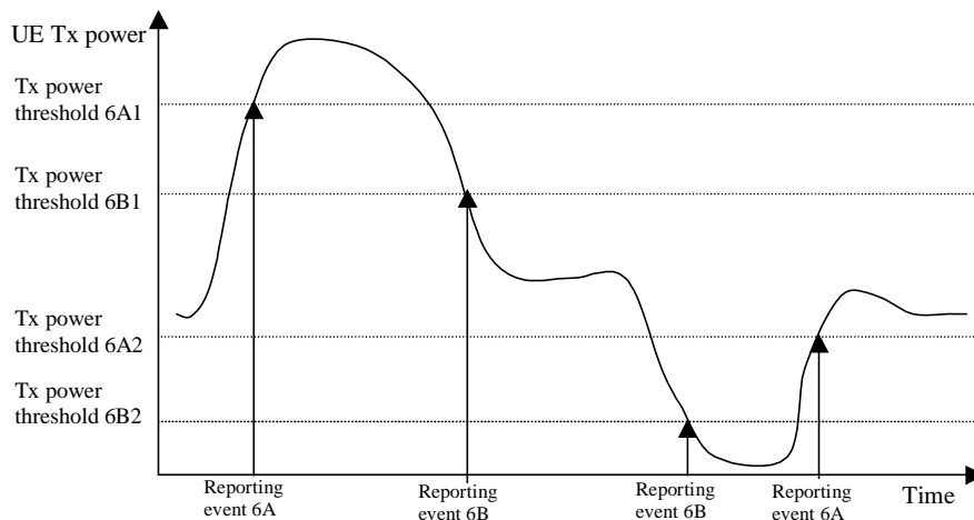
Figure 14.6.2.2-1: Event-triggered measurement reports when the UE Tx power becomes larger or less than absolute thresholds
