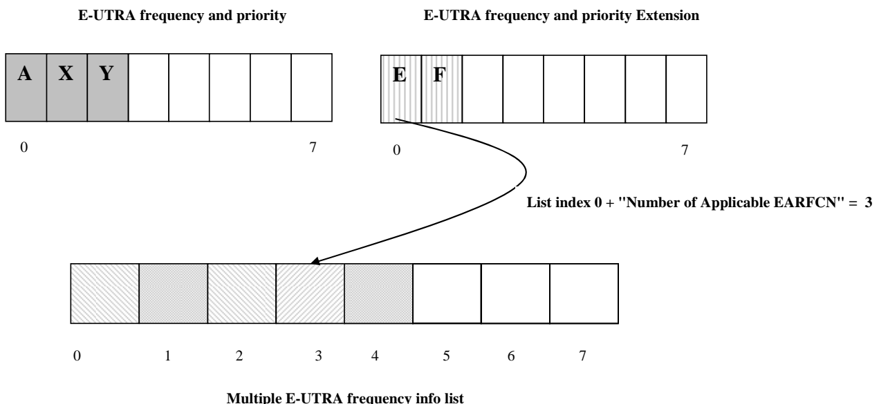
Figure: G.3.1 – Mapping of EARFCN's to Multiple E-UTRA frequency info list
