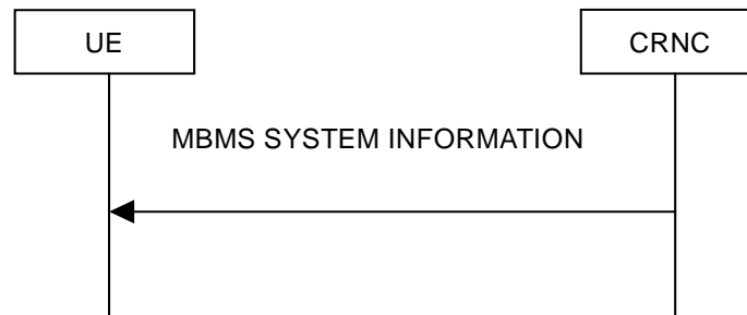
Figure 8.3.1: Broadcast of MBMS system information.
