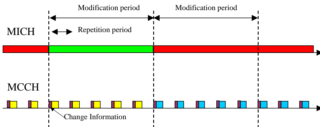
Figure 5.2.4: Illustration of MICH timing relative to Modification period
