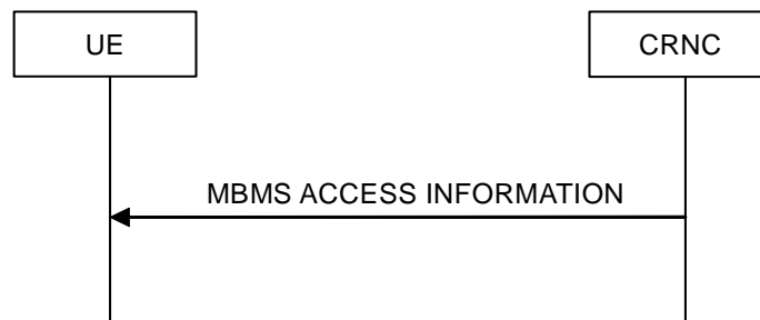
Figure 8.3.4: MBMS Access Information signalling flow
