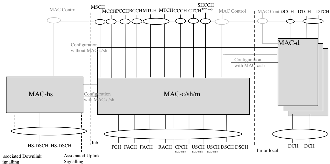
Figure 5.4.1: UTRAN MAC architecture
