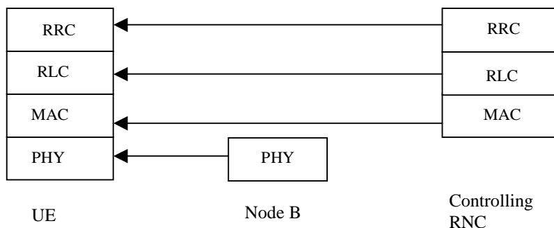
Figure 5.3.2: Protocol Stack for MCCH and MSCH
