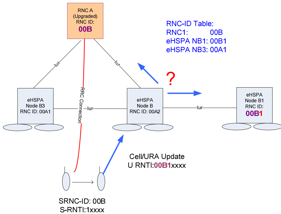
Figure A2.2.2.3: Problematic configuration example (does not follow Rule3)
