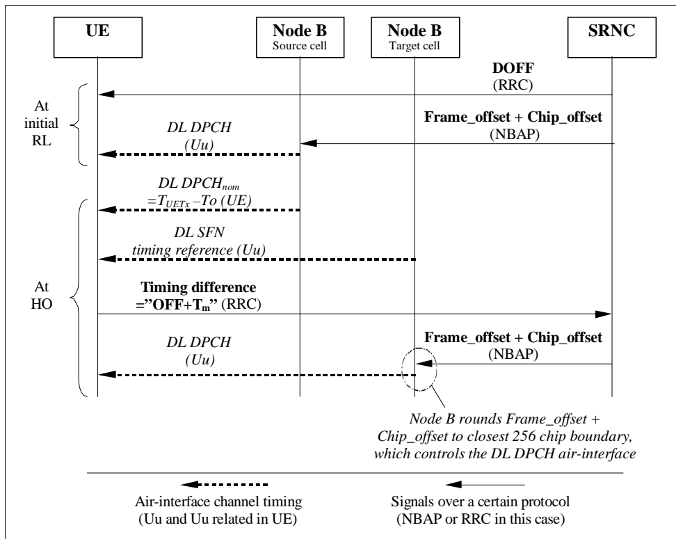
Figure 11: [FDD] Usage of Offset values at initial RL and at HO
