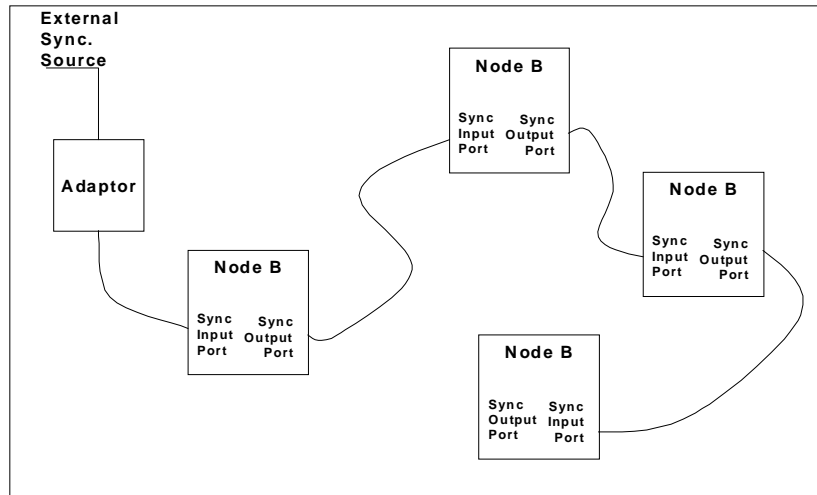
Figure 2: Usage of Synchronisation Ports
