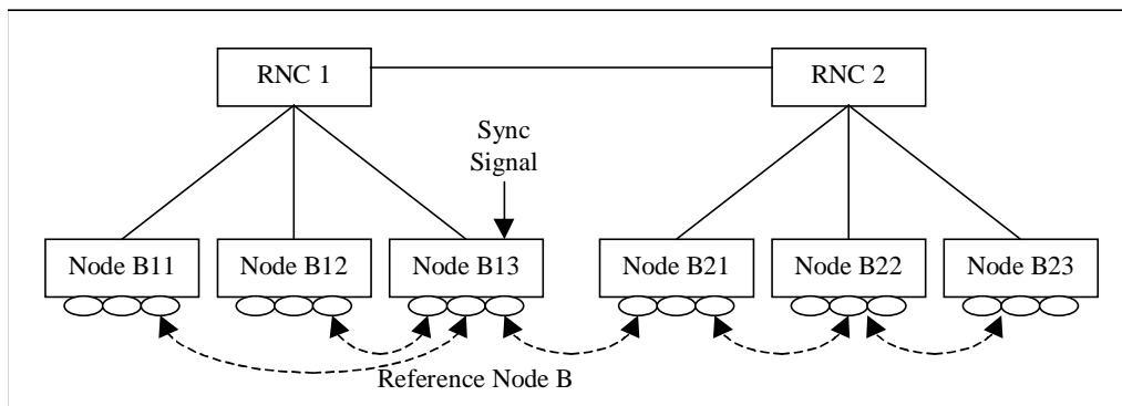
Figure 4: TDD Inter Node B Node Synchronisation
