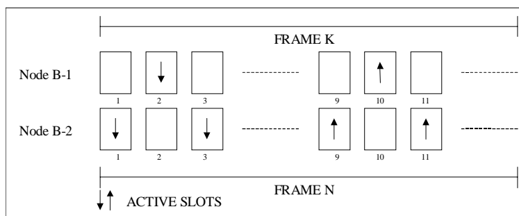
Figure 9: Radio Frame Synchronisation
