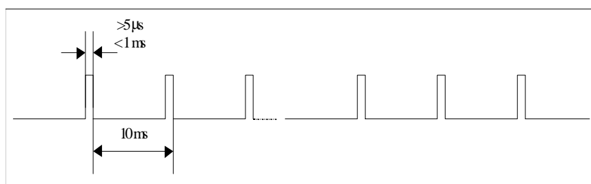
Figure 3: Synchronisation signal
