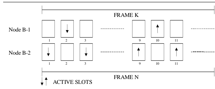
Figure 16: Intercell Synchronisation
