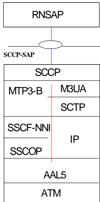
Figure 1: Signalling bearer for RNSAP
