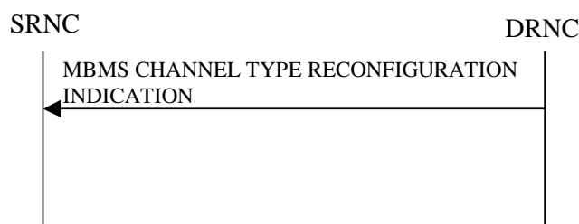
Figure 33: MBMS Channel Type Reconfiguration procedure, Successful Operation
