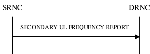
Figure 26R: Secondary UL Frequency Reporting procedure
