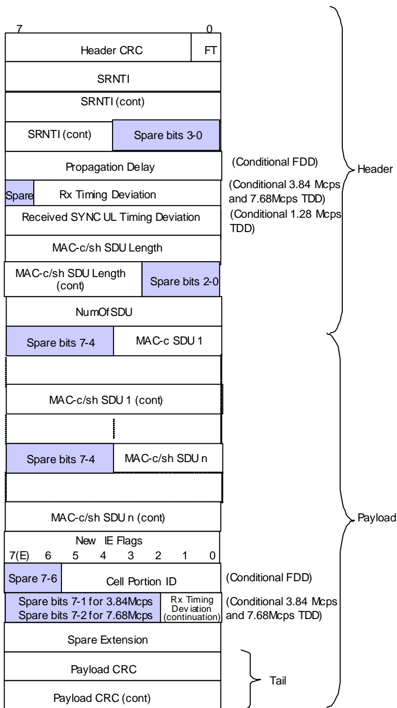
Figure 9: RACH DATA FRAME structure
