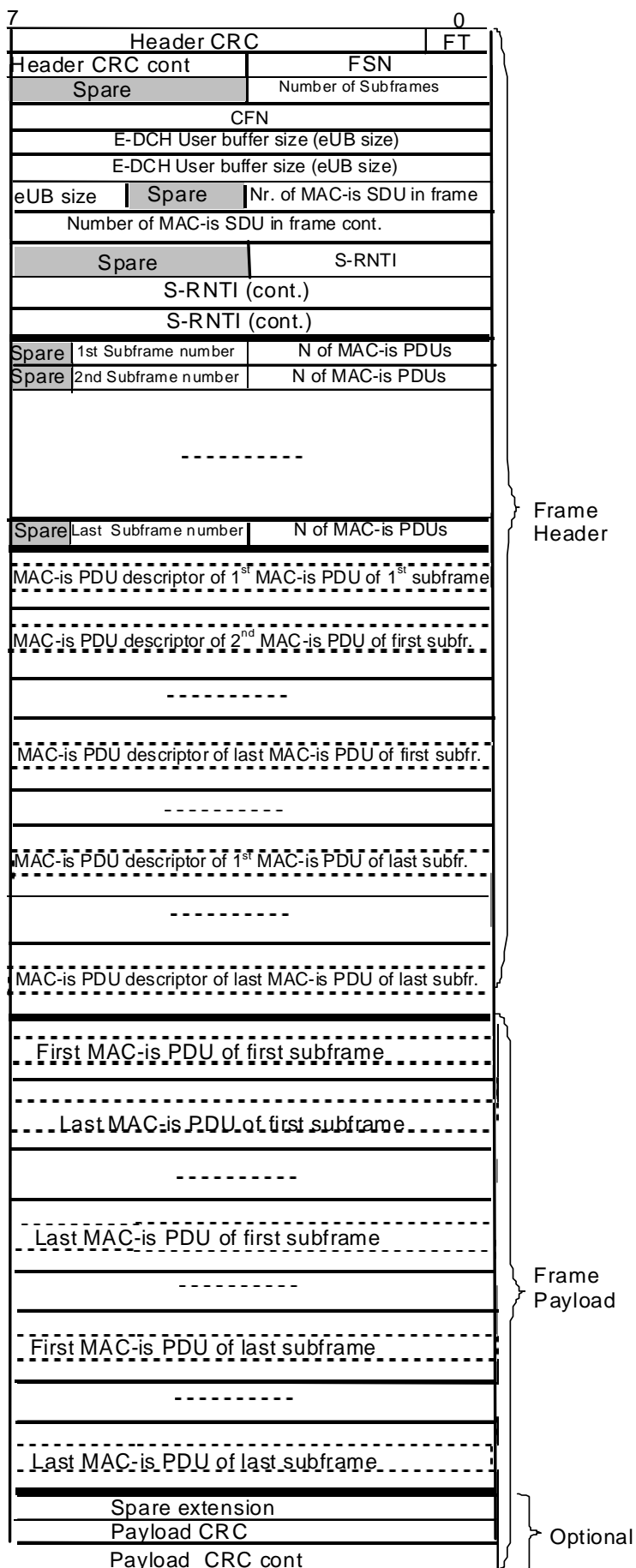
Figure 12C: E-DCH DATA FRAME structure
