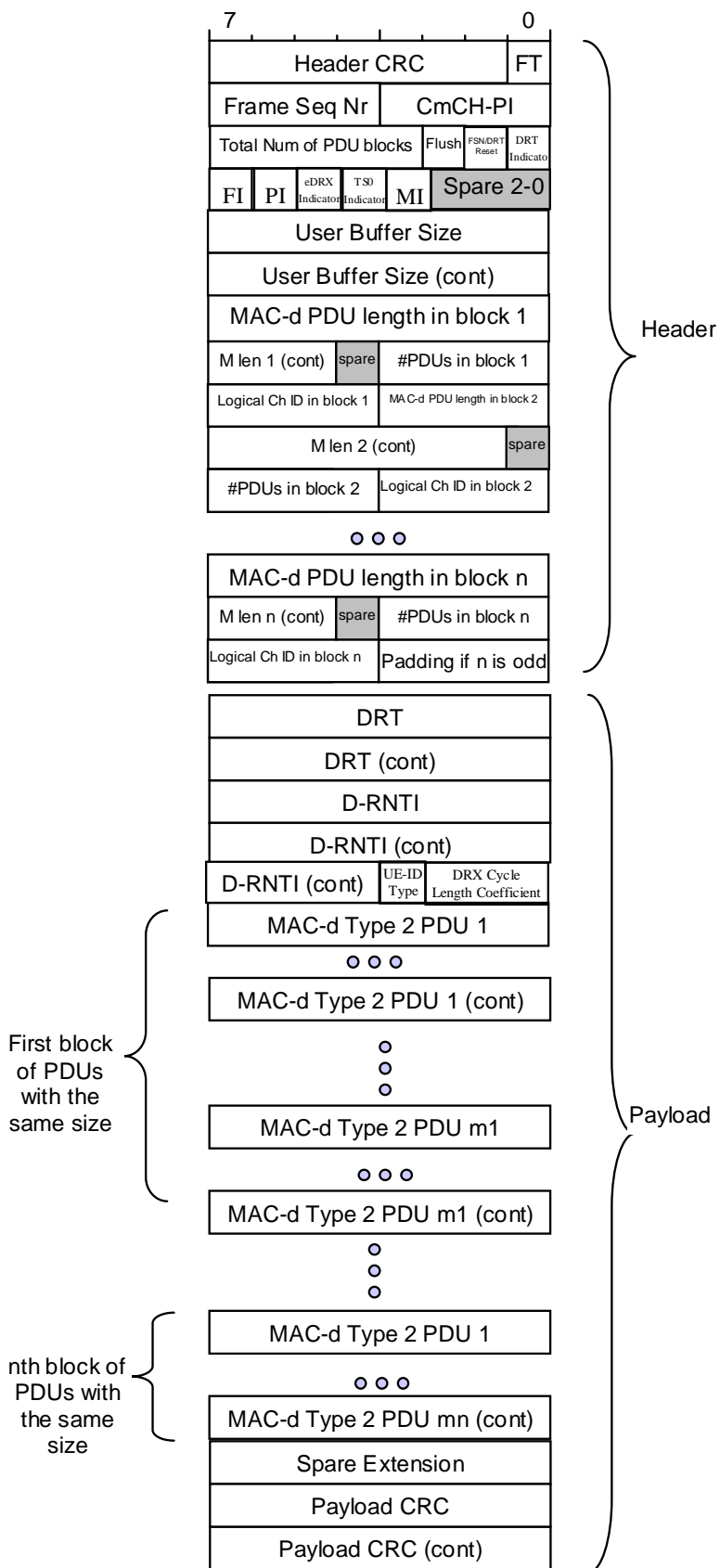
Figure 12B: HS-DSCH DATA FRAME TYPE 2 structure
