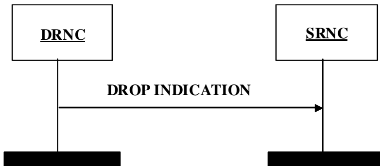
Figure 6E: HS-DSCH DROP INDICATION procedure
