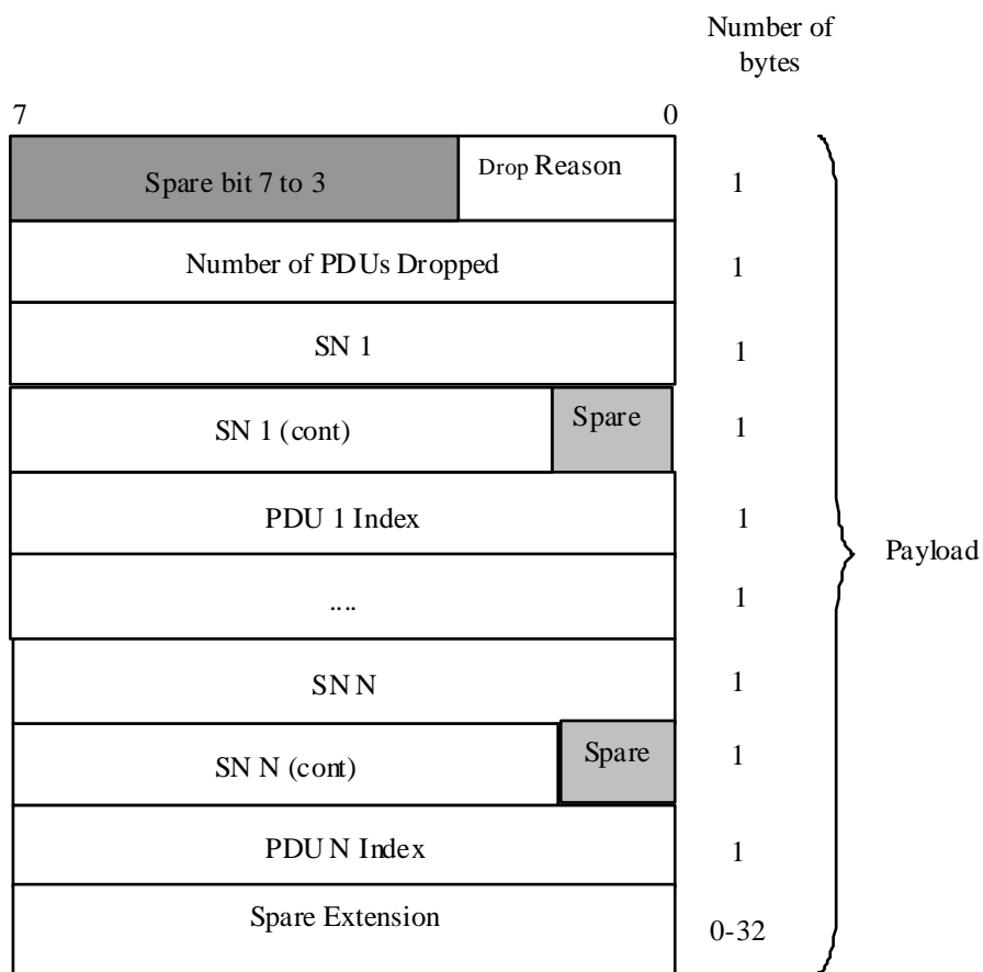
Figure 24: HS-DSCH DROP INDICATION payload structure
