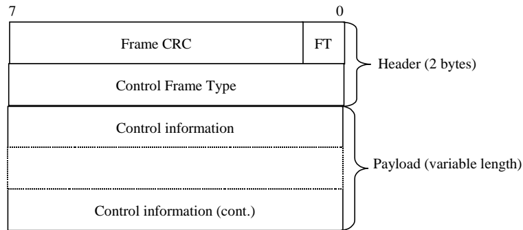
Figure 20: Iub Common Transport Channel Control Frame Format
