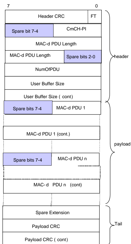
Figure 21A: HS-DSCH DATA FRAME structure
